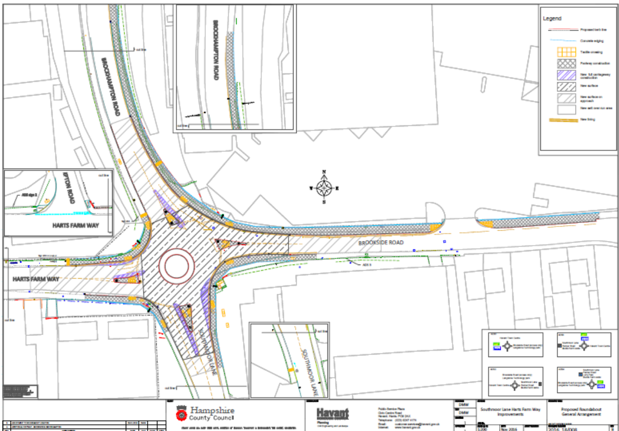
General Arrangement
